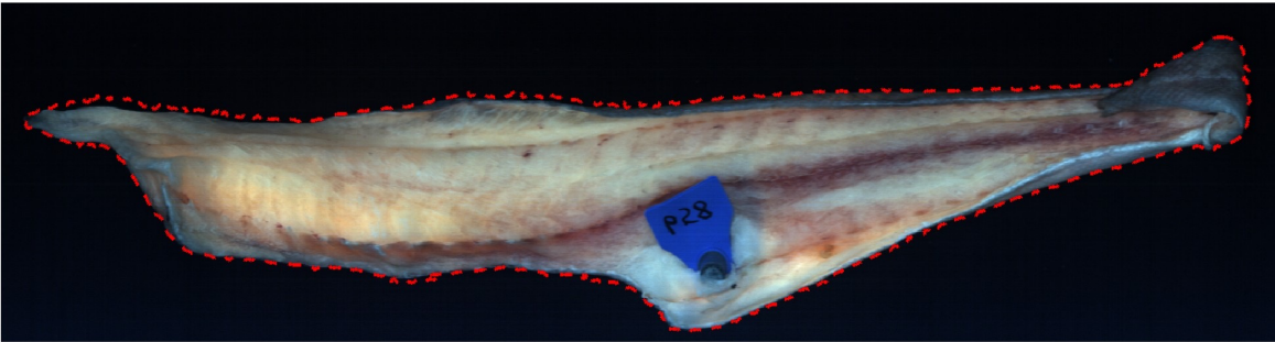
Sample 658 RGB False color
